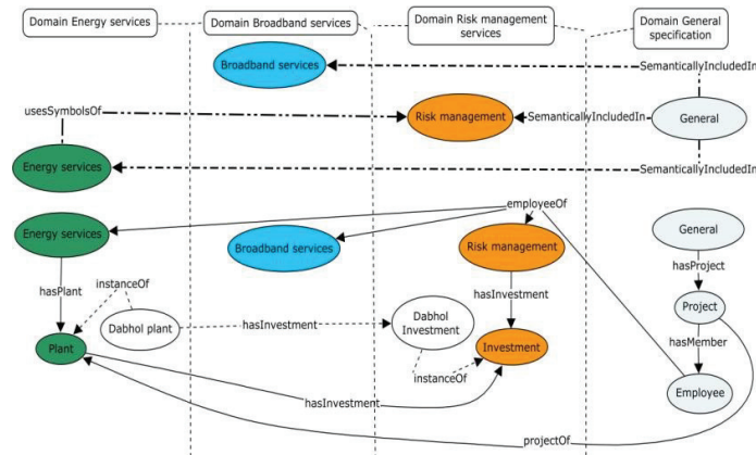
Fig. 3. Ontology Network
