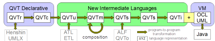
Fig. 1. Progressive transformation approach for Declarative QVT.
