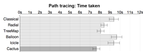
Fig. 6. Time taken (lower is better) for path tracing ( T2 ) for each of six layouts. CactusTree is highlighted in darker bars.
