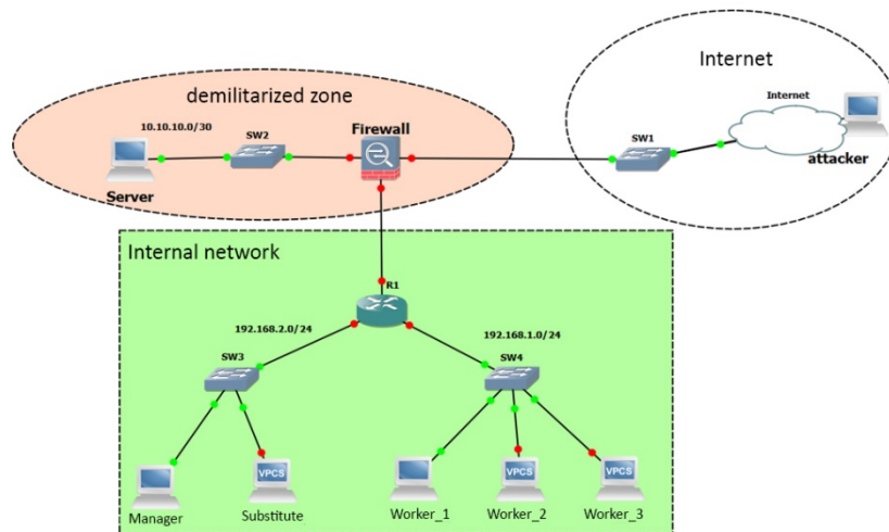
Fig. 1. Network topology in GNS3
