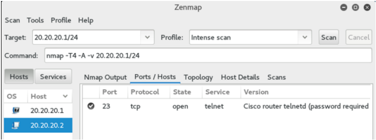
Fig. 4 Scan of Cisco 3745 Router with enabled Telnet
