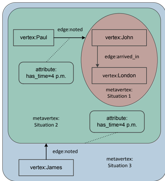
Figure 7 The metagraph representation of RDF reification
