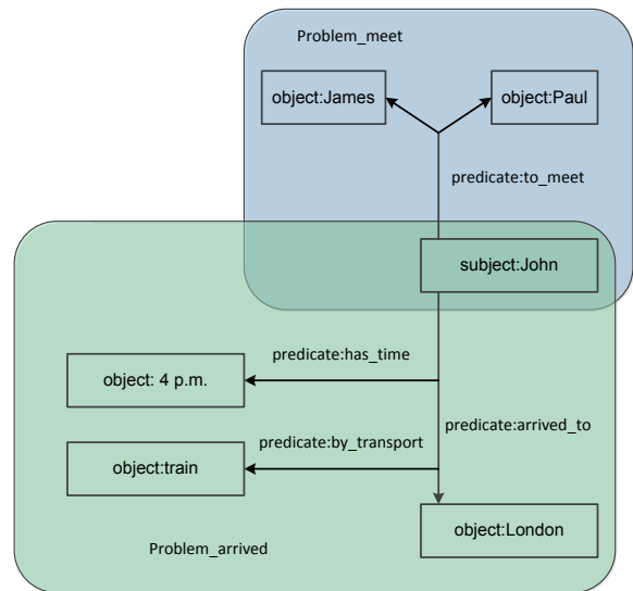
Figure 8 The example of N-ary relationship
