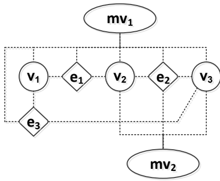
Figure 3 The example of flattened metagraph
