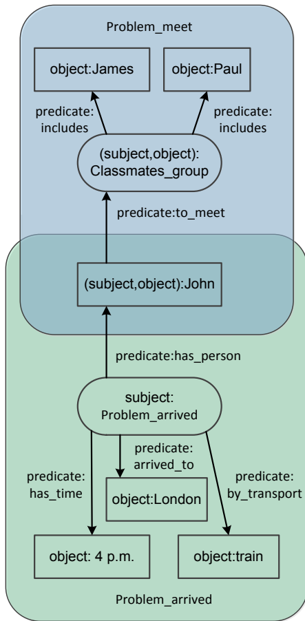
Figure 9 The RDF representation of N-ary relation example
