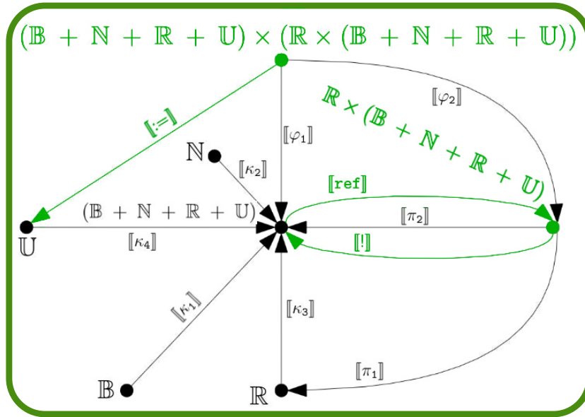
Fig. 3. Categorical model of reference type
