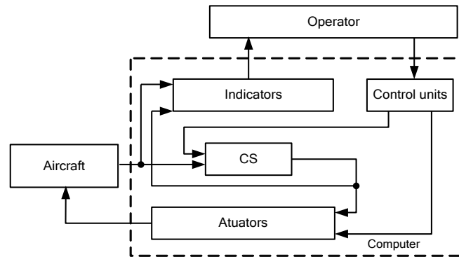
Fig. 2. Structure of the human-machine system of the second type (CS is a control system)
