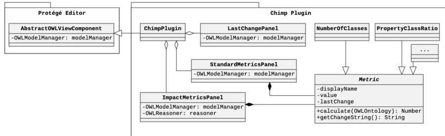
Fig. 5: UML Class diagram of the ChImp implementation, showing its architecture.
