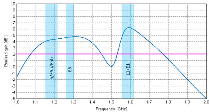
Figure 10. Peak realized antenna gain of designed Crossed IFAs antenna.
