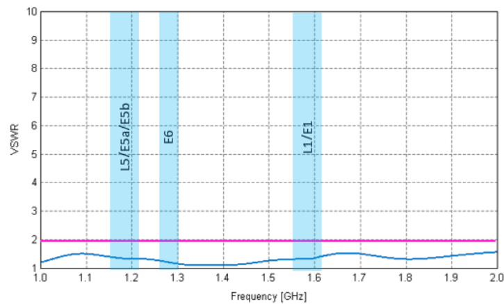
Figure 6. VSWR of designed Crossed IFAs antenna
