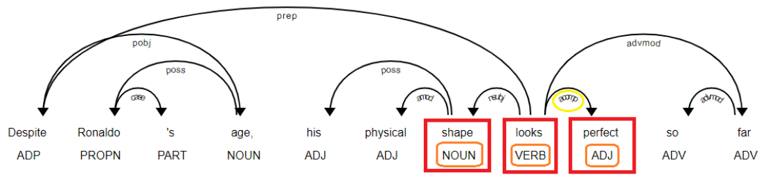
Figure 1: An illustration on the focused fragment of text for the sentence: Despite Ronaldo's age, his physical shape looks perfect so far.
