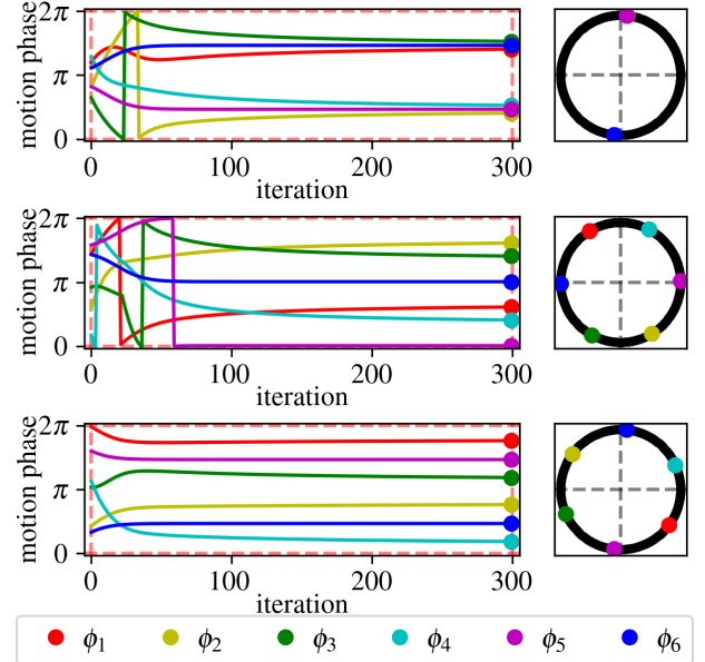
Figure 9: On the left: the first 300 iterations of \phi_i self-organizing motion phases, where the vertical axis represents the value of the motion phase at each iteration given by the horizontal axis. On the right: the final positions at the 20000-th iteration of the organized motion phases, depicted as a unit circle using \cos(\phi) for horizontal axis and \sin(\phi) for vertical axis for \phi \in [0, 2\pi) (compare with desired patterns in Fig. 2). The plots correspond to the tripod, transition, and wave gaits from top to down, respectively. Note that motion phases for simultaneously activated legs in the tripod gait are overlapping.
