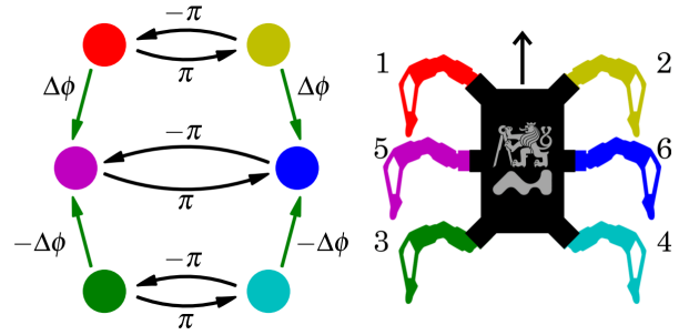
Figure 1: On the left: schema of leg motion phase \phi_i relations. Each vertex represents the motion phase of the leg of the corresponding color on the corresponding anatomic position. The black oriented edges indicate repulsive forces maintaining antiphase; the green edges indicate keeping a specified distance from the other phase. The colors and positioning correspond to the robot schema on the right. On the right: the robot schema with colored and labeled legs, corresponding to labeling in Figs. 2 and 3. The arrow indicates the direction of the robot's movement.
