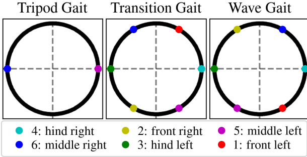
Figure 3: Example visualization of motion phases \phi_i (colorful dots) correctly ordered within the phase (black circle) to produce the desired gait patterns. The interval [0, 2\pi) representing phase is depicted as a unit circle using \cos(\phi) for the horizontal axis and \sin(\phi) for the vertical axis for \phi \in [0, 2\pi) . Note that the ordering and relative distance (phase offset) of actions are important, not their particular position within the phase. The gaits have more valid ordering options, and the figure represents only one of the possible orderings. The motion phases for simultaneously activated legs in tripod gait are overlapping.
