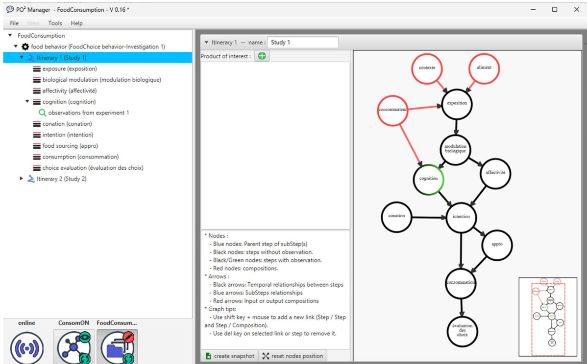
Figure 2: PO 2 Manager screenshot displaying a Food Consumption process implementation (note that this is a preliminary version subject to change). A red node is an input or output component (po2:Component), a black node is a step of the process (po2:Step), and a back/green node is a step that contains data tables (sosa:ObservationCollection).
