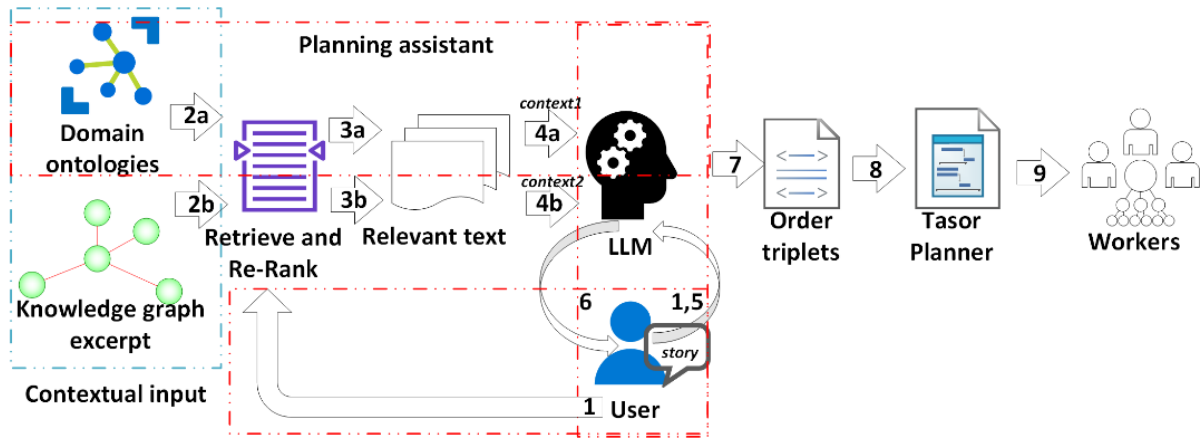
Figure 2: LLM-aided planning workflow: 1,5-User input {story} 2a-RDF schema 2b-RDF knowledge graph 3a-Ontology chunks 3b-Knowledge graph excerpt chunks 4a-Context: ontology excerpt {context1} 4b-Context: knowledge graph template {context2} 6-Intermediary result 7-Triplets 8-Order definition 9-Generated work plan.
