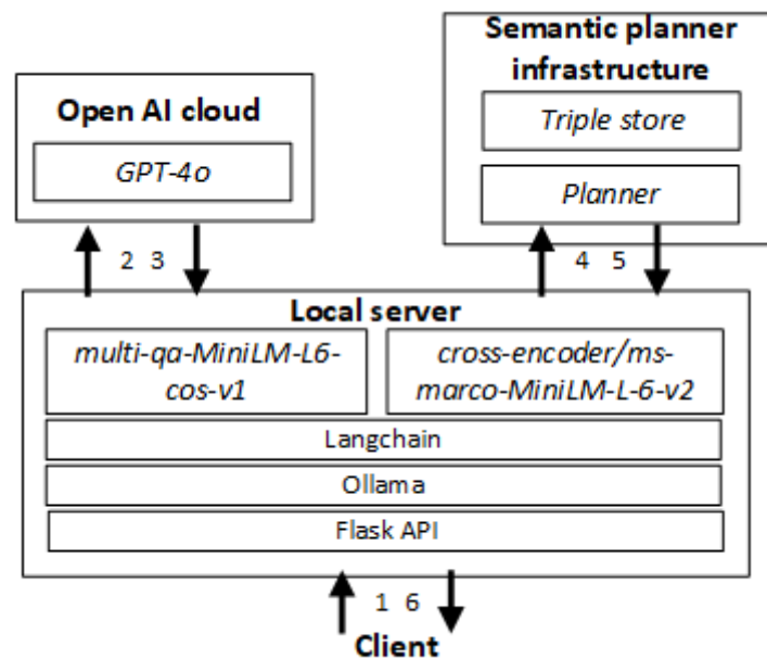
Figure 3. Deployment overview: 1-HTTP request containing user story; 2-Prompt to GPT-4o; 3-Response of GPT-4o; 4-Triplet insertion; 5-Planning output; 6-HTTP response (created triplets/plan).
