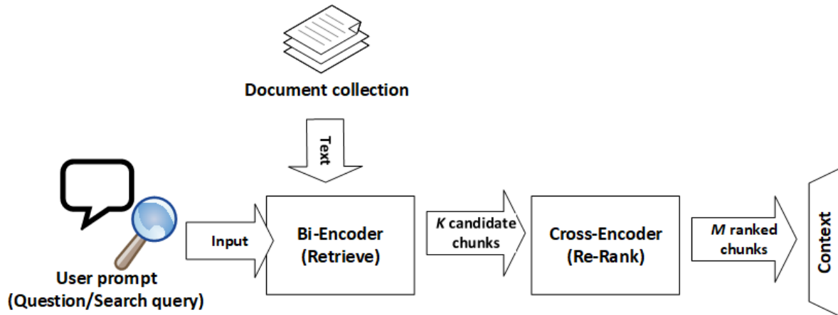
Figure 1: Retrieve and Re-Rank for In-Context Learning (RRR4ICL) approach workflow overview, K > M .
