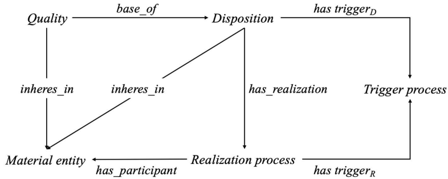
Figure 1: The relations between the classes disposition , material entity , quality , and realization and trigger processes in the Röhl–Jansen pattern (our diagram based on [7]).
