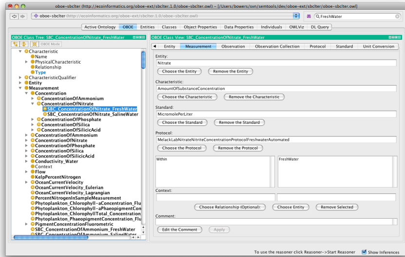
Fig. 2. The Measurement form showing the various fields of a “Fresh Water Nitrogen Concentration” measurement type defined within the an OBOE extension ontology.
