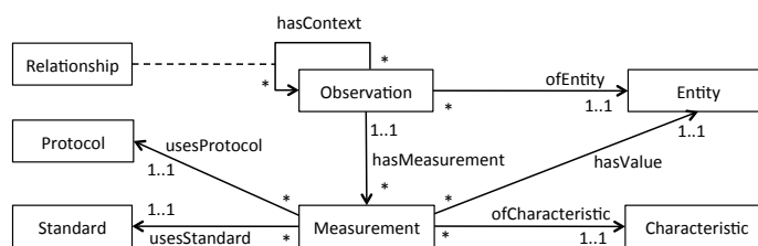
Fig. 1. The main classes and properties of the observation and measurement ontology (OBOE). While shown in UML, the model is defined using OWL-DL.
